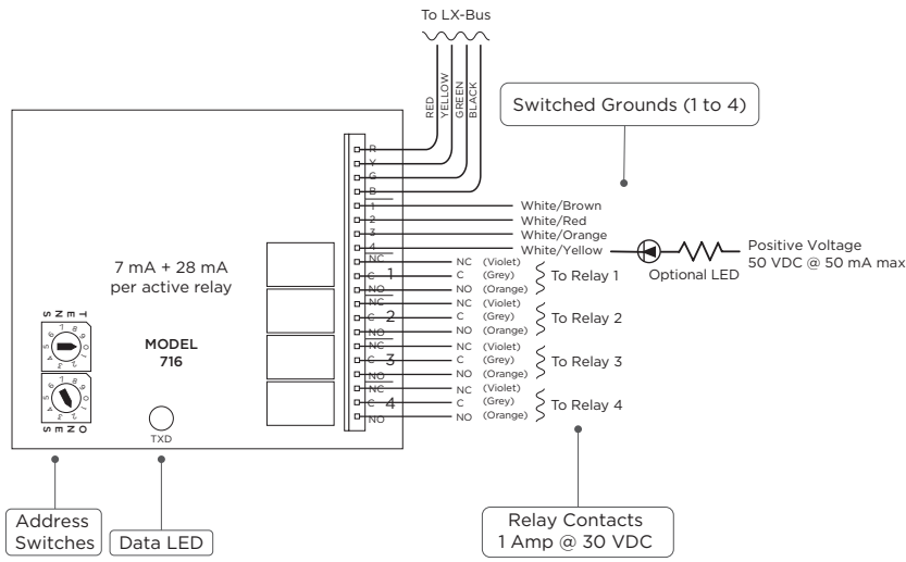
Figure 4: Module Wiring
