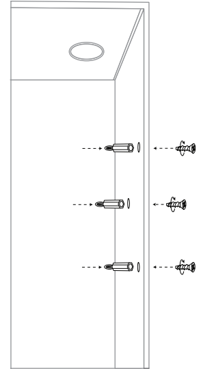
Figure 2: Standoff Installation
