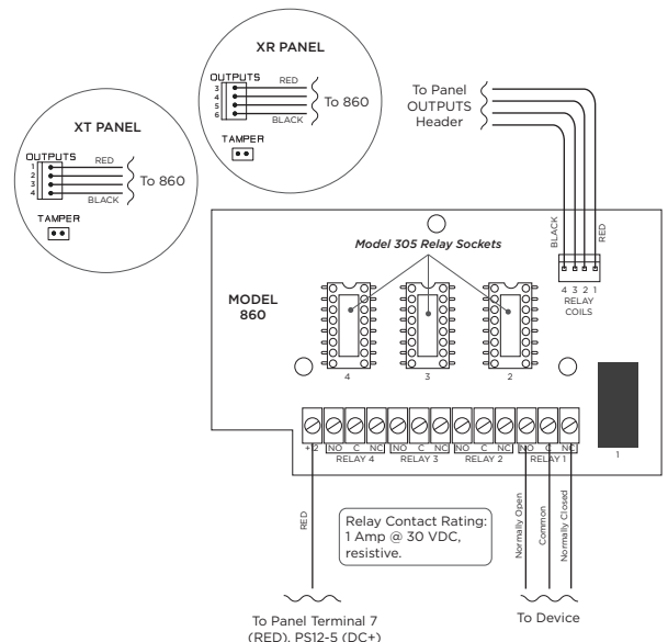
Figure 3: Wiring Connections
