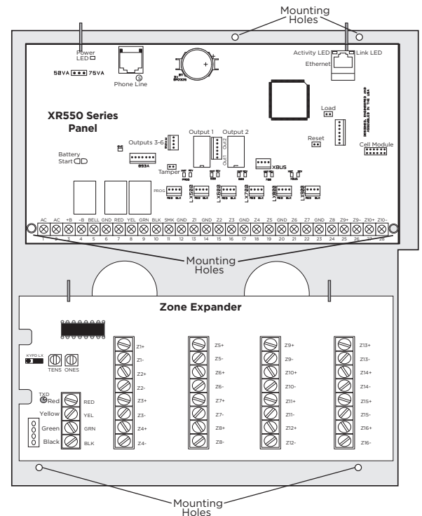
Figure 1: Mounting Plate with Panel and Zone Expander
