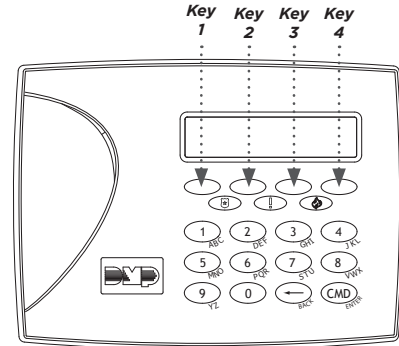
LCD Keypad Select Keys
