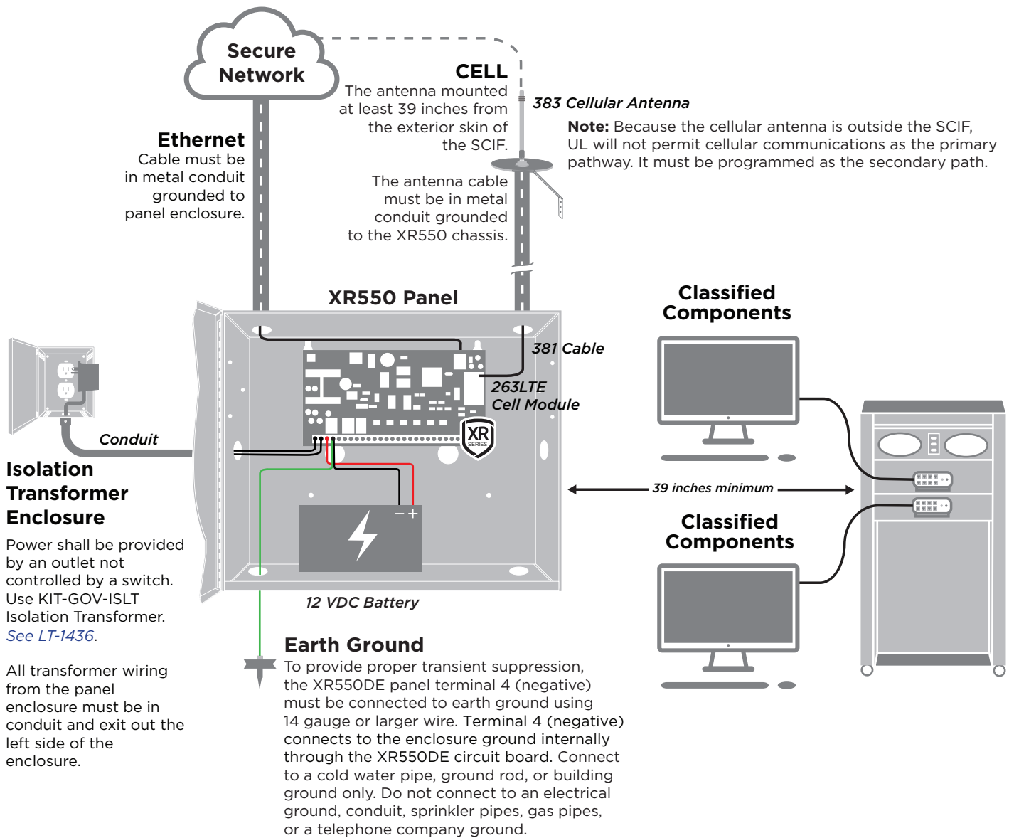
Figure 1: SCIF Setup Diagram
