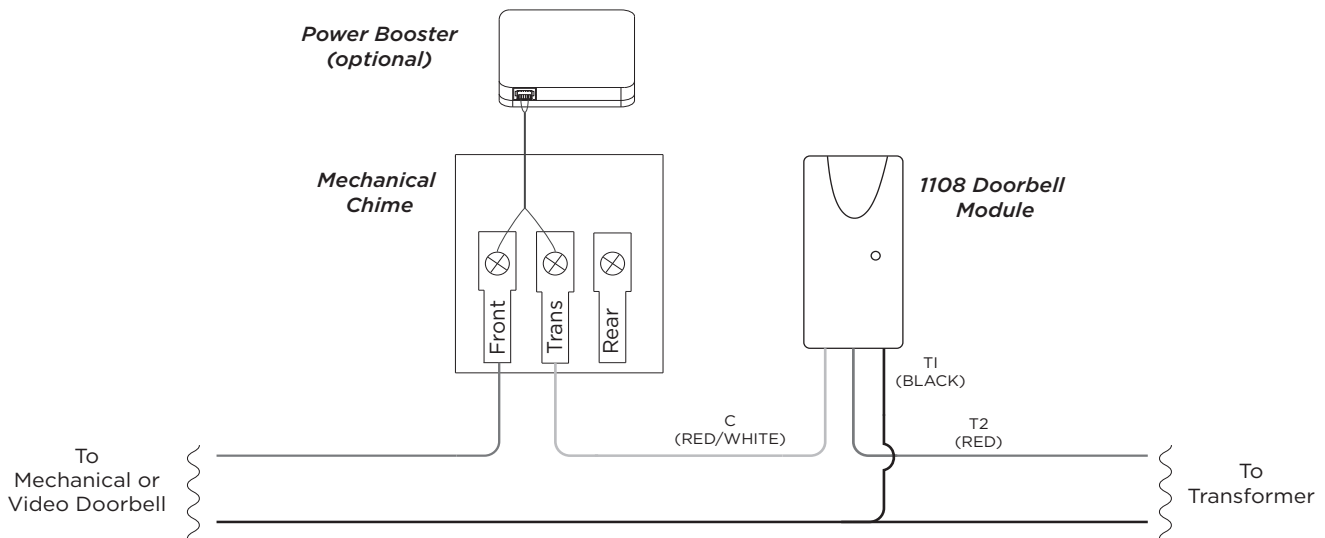
Figure 3: 1108 Wiring with Existing Chime
