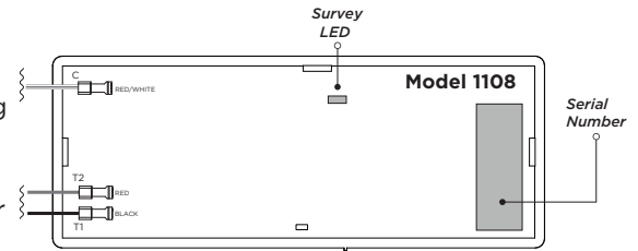
Figure 2: PCB Features
