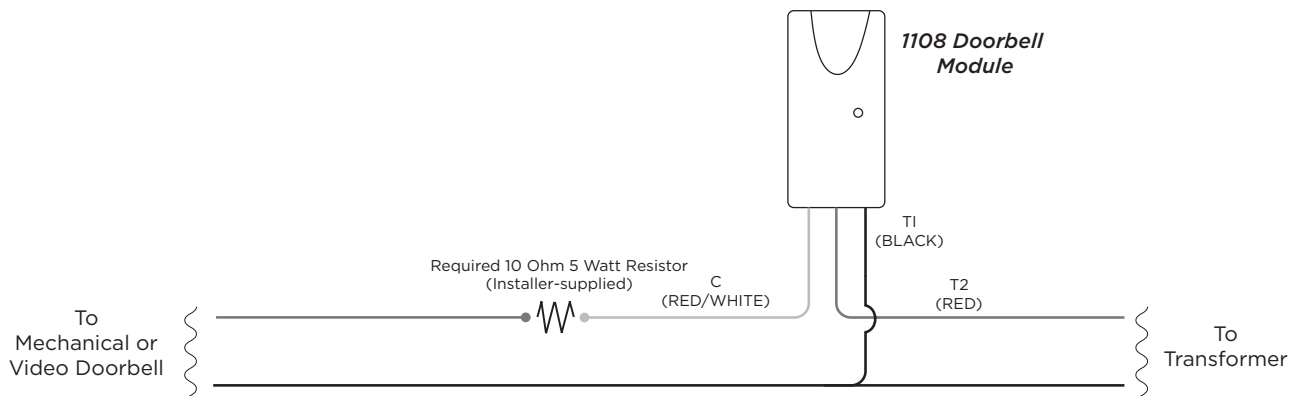
Figure 4: 1108 Wiring without Chime
