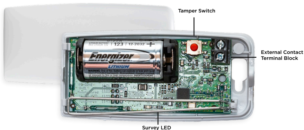
Figure 1: 1101 Layout
