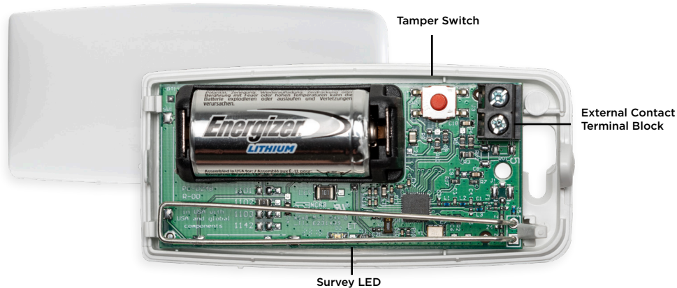
Figure 1: 1102 Layout
