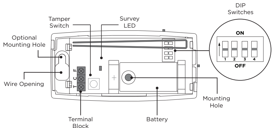
Figure 2: Transmitter Components
