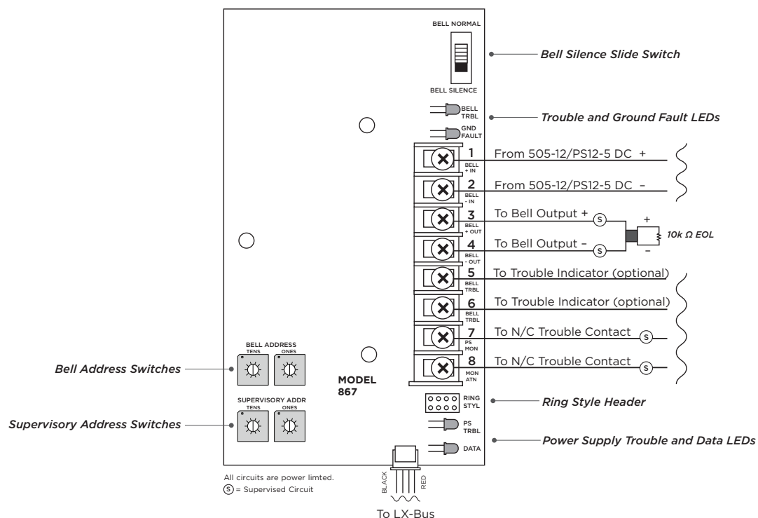
Figure 3: Wiring Connections
