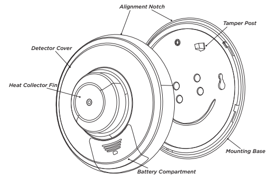
Figure 5: Heat Detector Exploded View
