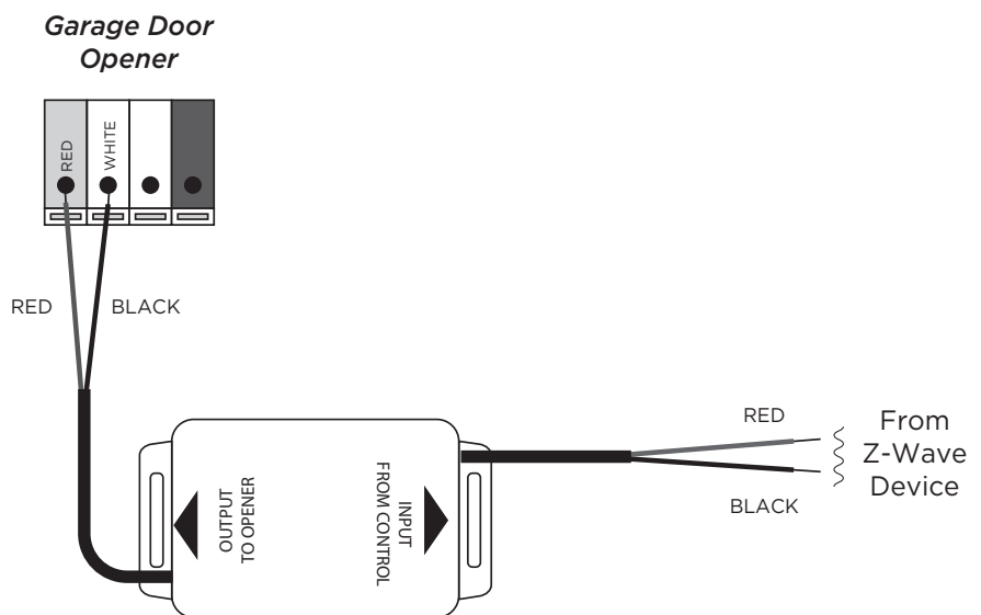
Figure 2: 736Q Wiring
