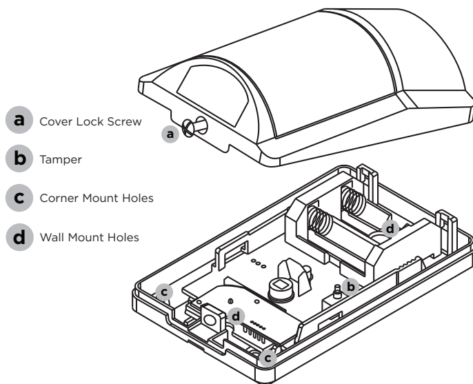
Figure 3: Remove the Cover
