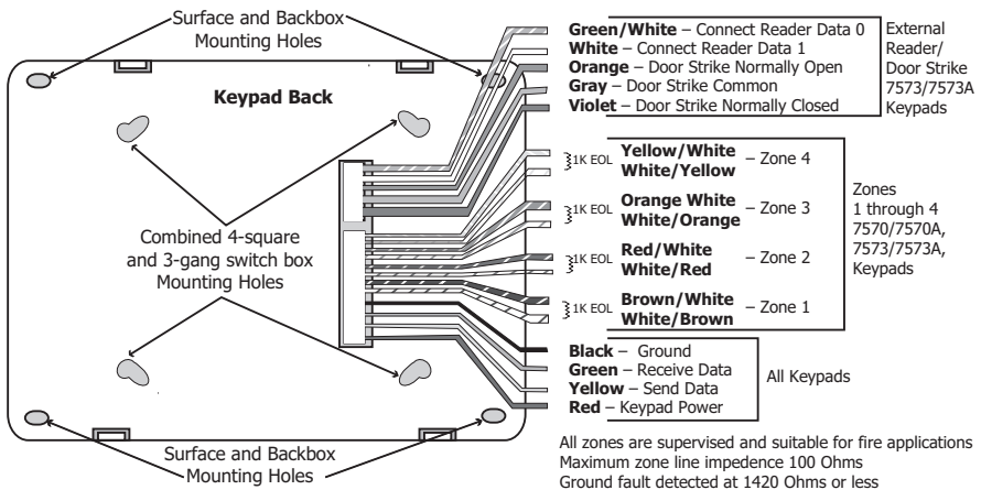
Figure 1: Keypad Back Showing Wiring Harness Assignments
