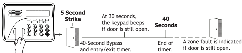
Figure 7: Door Strike Relay Operation Time Line
