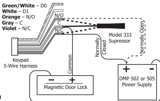
Figure 3: 5-wire Harness/Suppressor Installation
