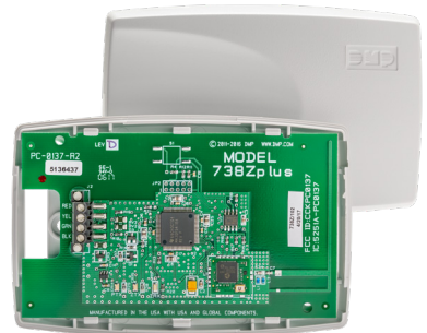
Figure 1: 738Zplus Z-Wave Interface Module
