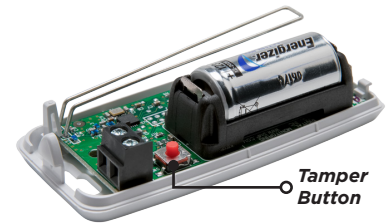
Figure 1: New 1103 Tamper Button
