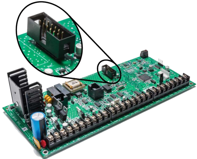
Figure 1: XT Series Panel with a Cell Pin Header Shroud
