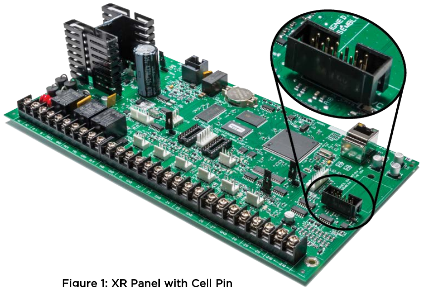
Figure 1: XR Panel with Cell Pin Header Shroud
