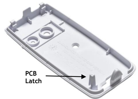
Figure 2: PCB Latch
