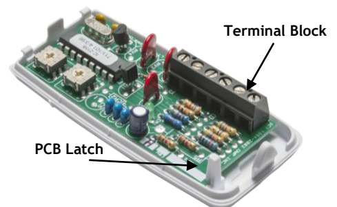
Figure 2: 711 PCB
