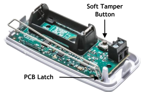
Figure 2: PCB Latch and Soft Tamper Button
