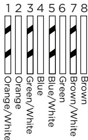
Figure 15: Cat 5 568-B Wiring
