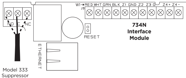
Figure 8: 333 Suppressor Installation
