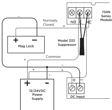
Figure 6: Magnetic Lock with an Isolation Relay
