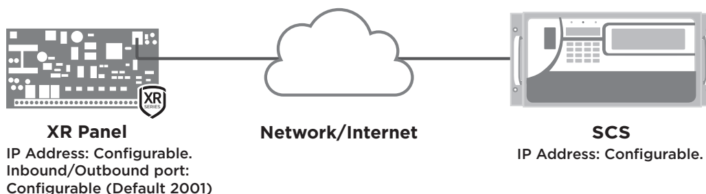
Figure 3: XR Series and SCS-1R Receiver
