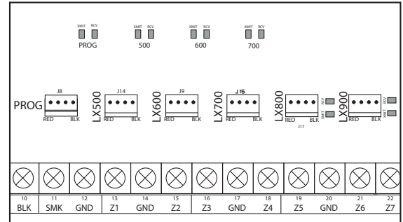
LX-Bus Headers and LEDs
