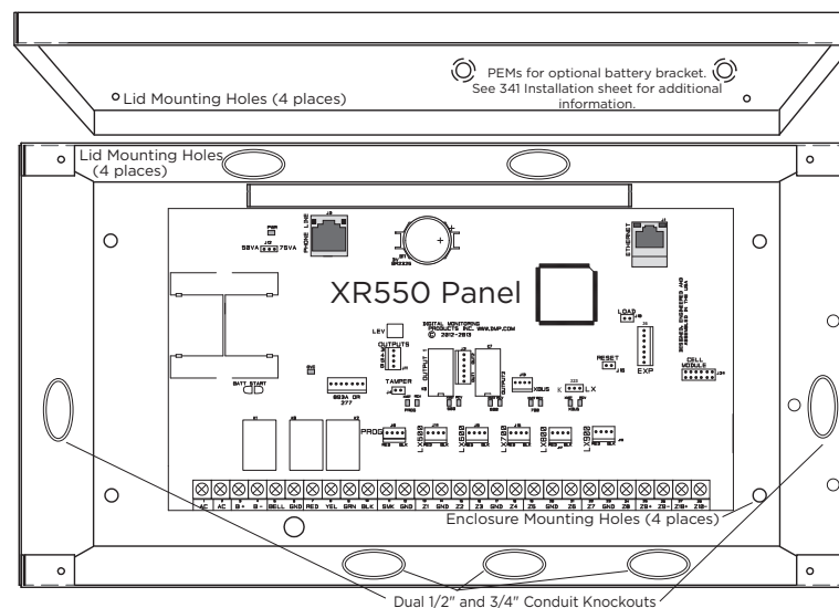
XR550 Series in Model 341 Enclosure
