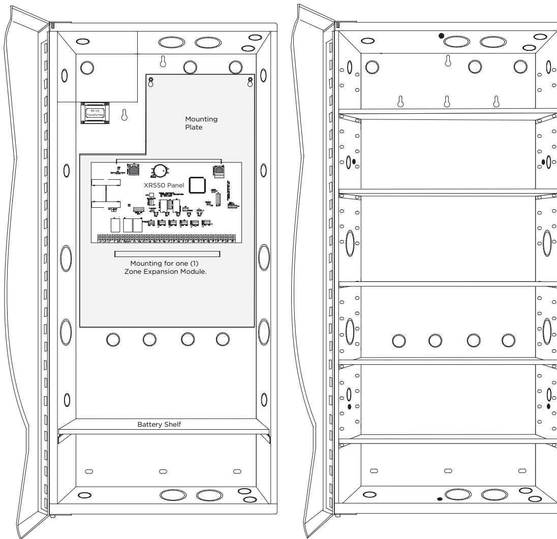
XR550 Series in Model 352X Enclosure and Separate 352S Enclosure with Shelves
