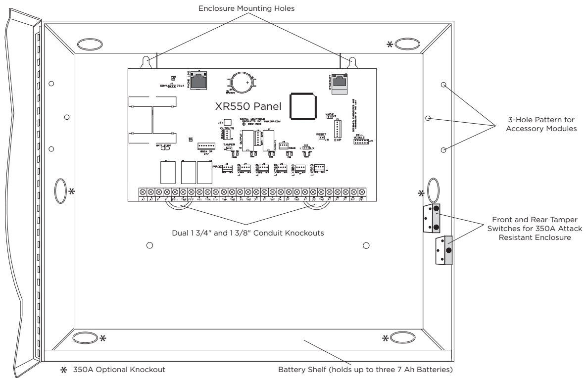
XR550 Series in Model 350 or 350A Enclosure
