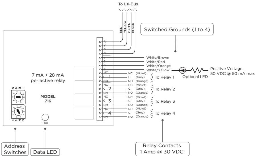
Figure 4: Module Wiring
