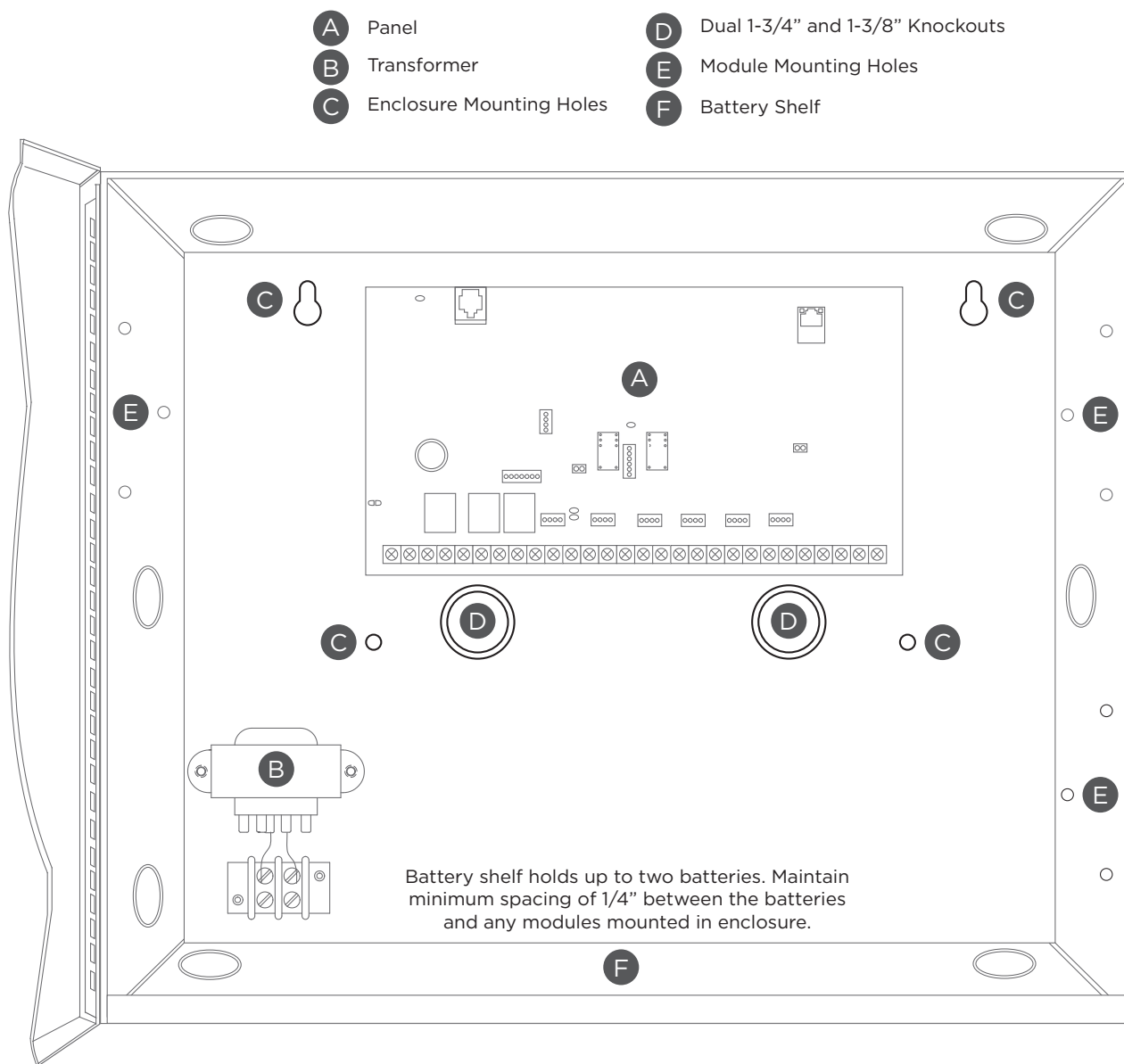
Figure 3: XR150FC/XR550FC Enclosure
