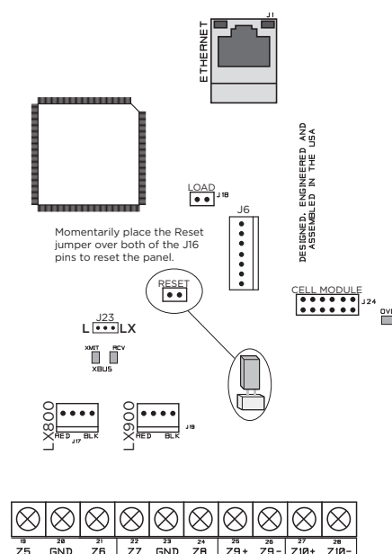
Figure 9: XR550FC Series Panel Showing the RESET Jumper
