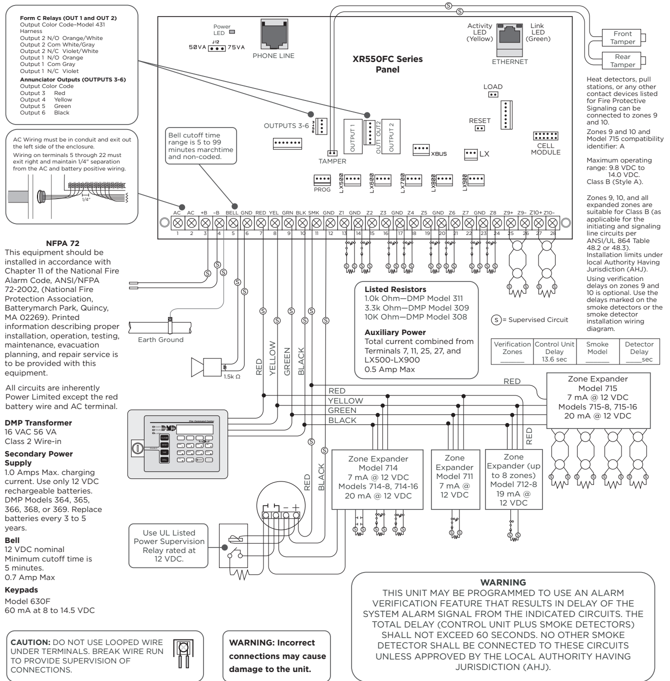
Figure 2: XR150FC/XR550FC Series Wiring Diagram
