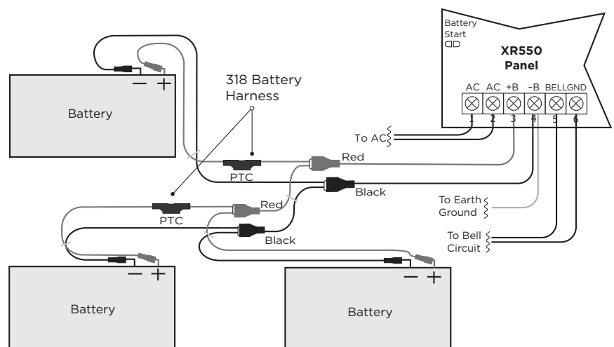
Figure 1: Wiring Multiple Batteries
