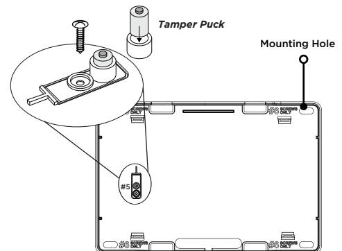
Figure 1: Inside of the 1100R Housing
