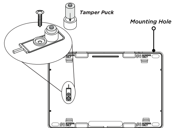
Figure 1: Inside of the 1100X Housing
